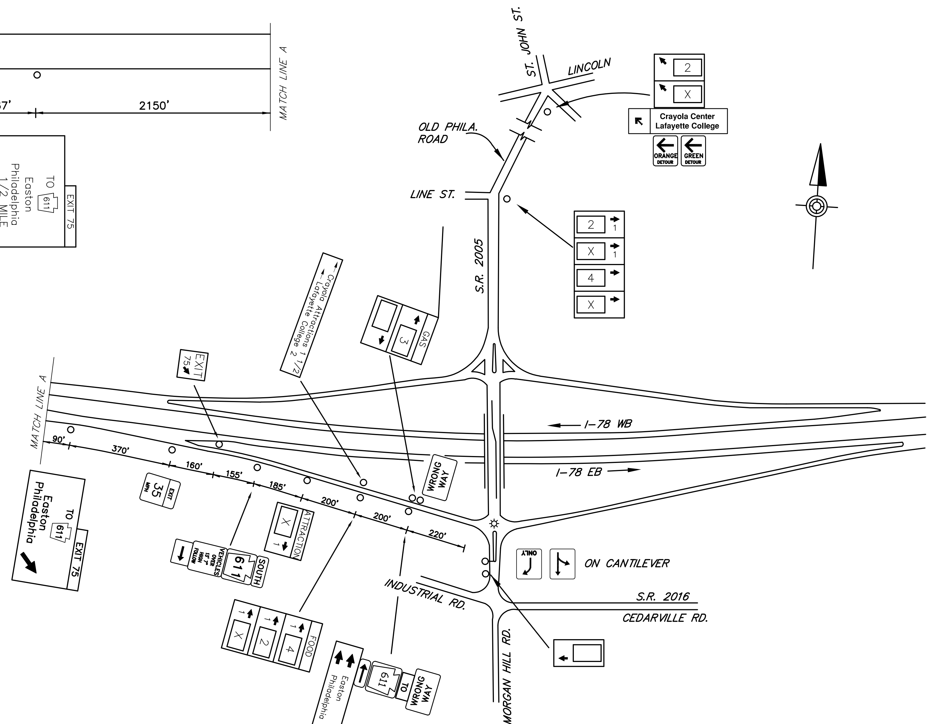
SCHEMATIC PLAN NOT TO SCALE
