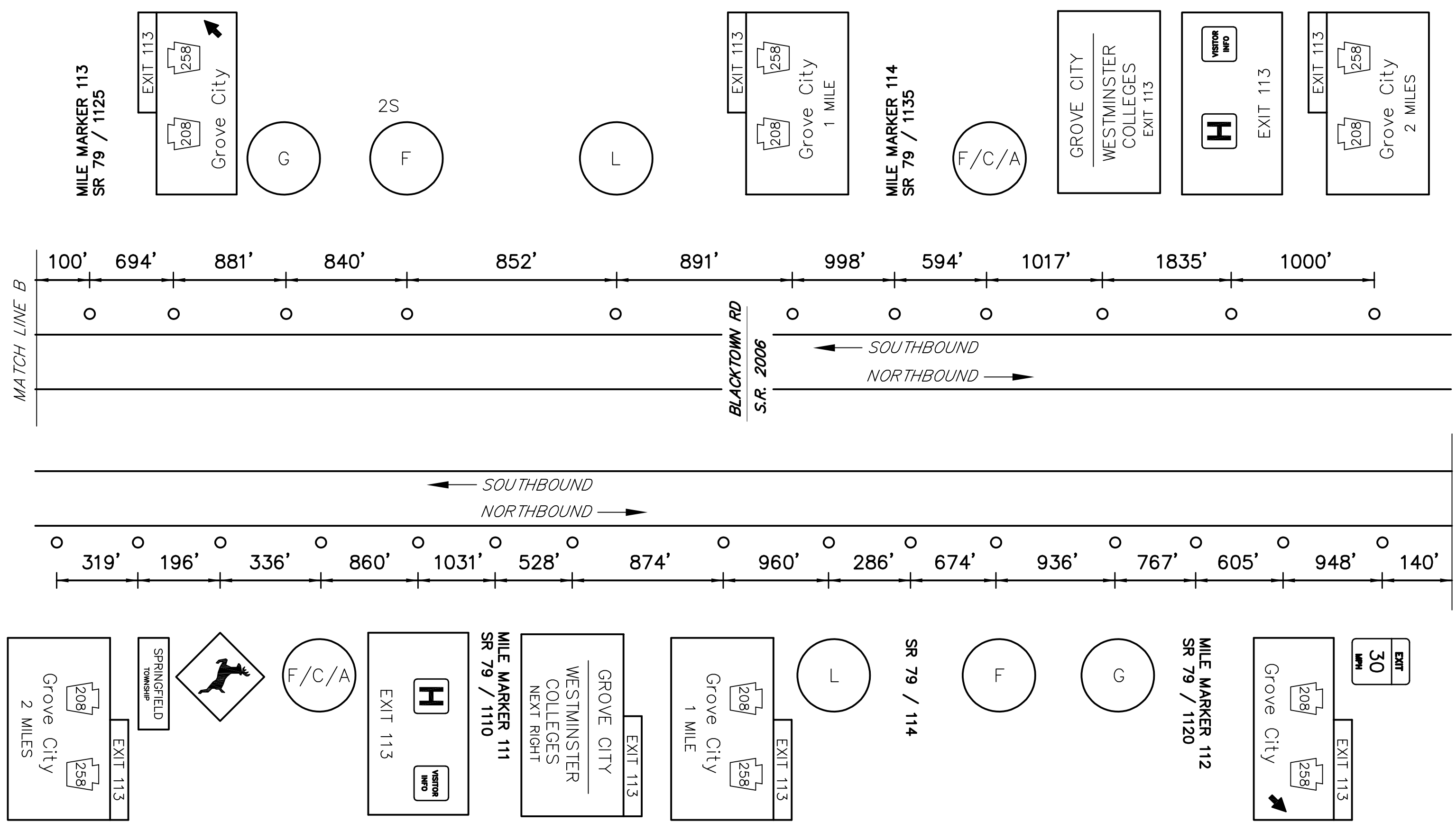
MAINLINE SCHEMATIC NOT TO SCALE
