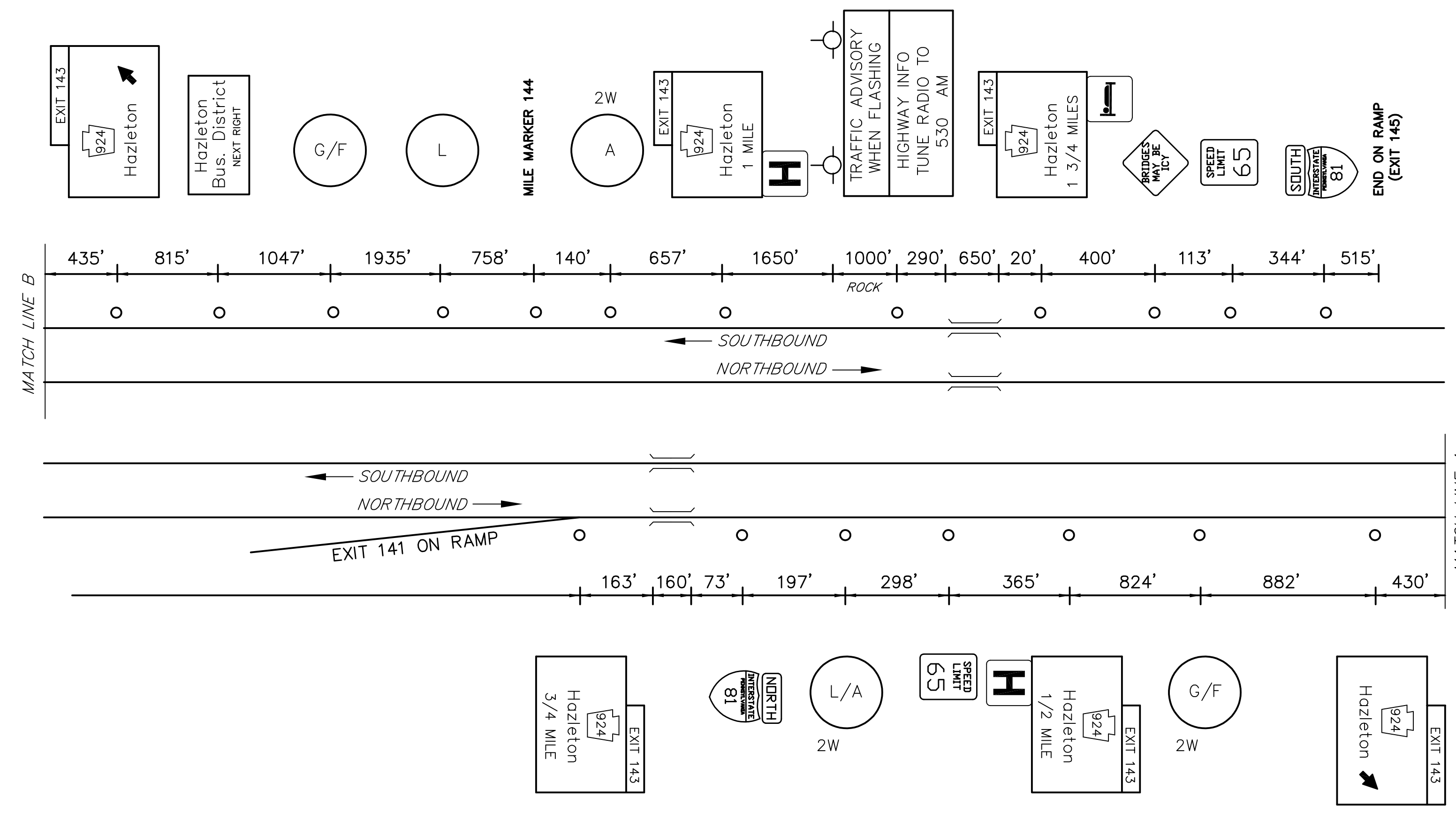
MAINLINE SCHEMATIC NOT TO SCALE
