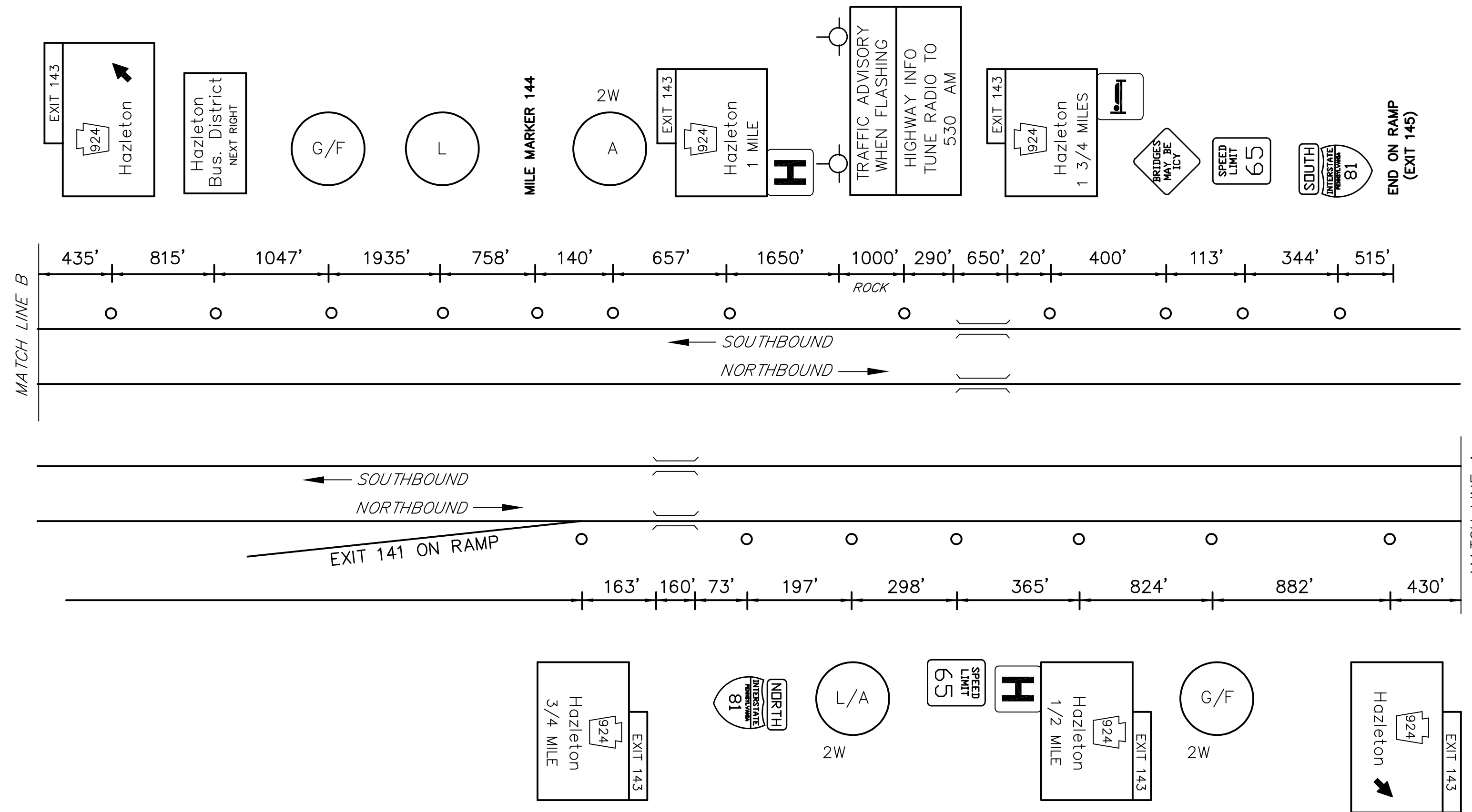
MAINLINE SCHEMATIC NOT TO SCALE
